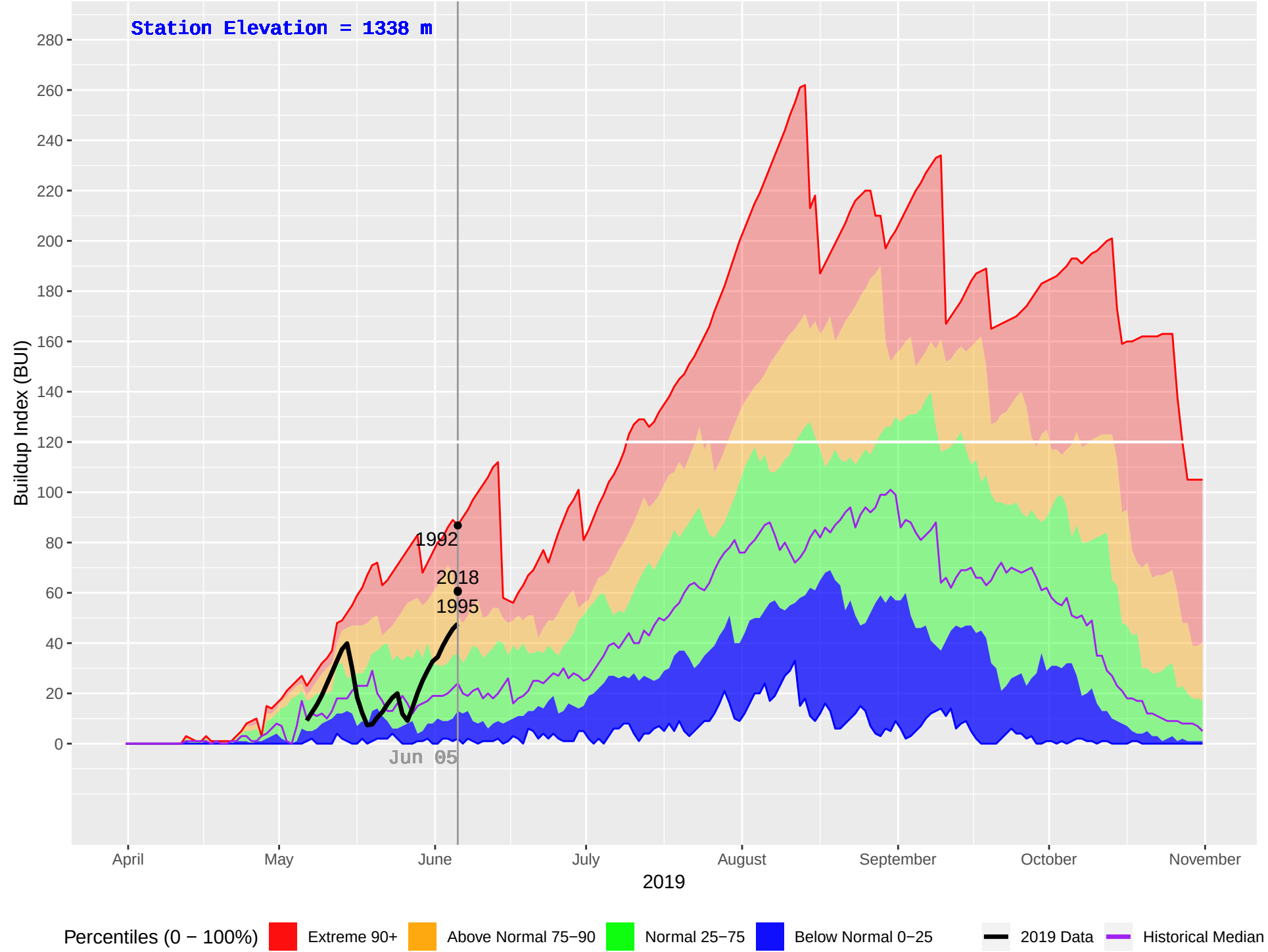
EIGHT MILE (391) : Historical (1980–2018), Current (2019) Daily Buildup Index (BUI)
