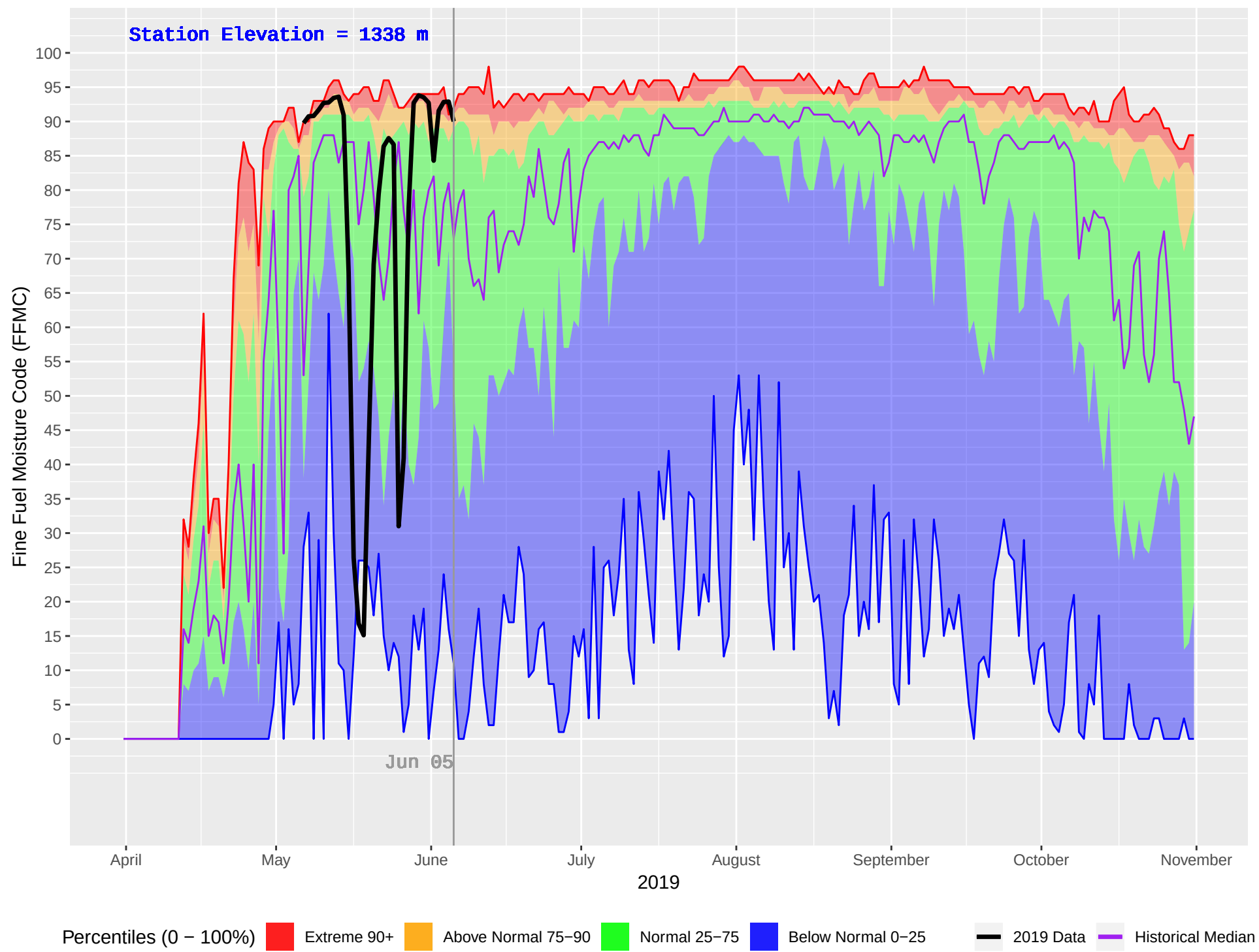
EIGHT MILE (391) : Historical (1980–2018) and Current (2019) Daily Fine Fuel Moisture Code (FFMC)
