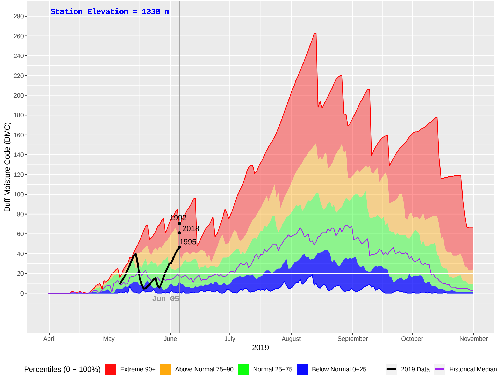
EIGHT MILE (391) : Historical (1980–2018), Current (2019) Daily Duff Moisture Code (DMC)
