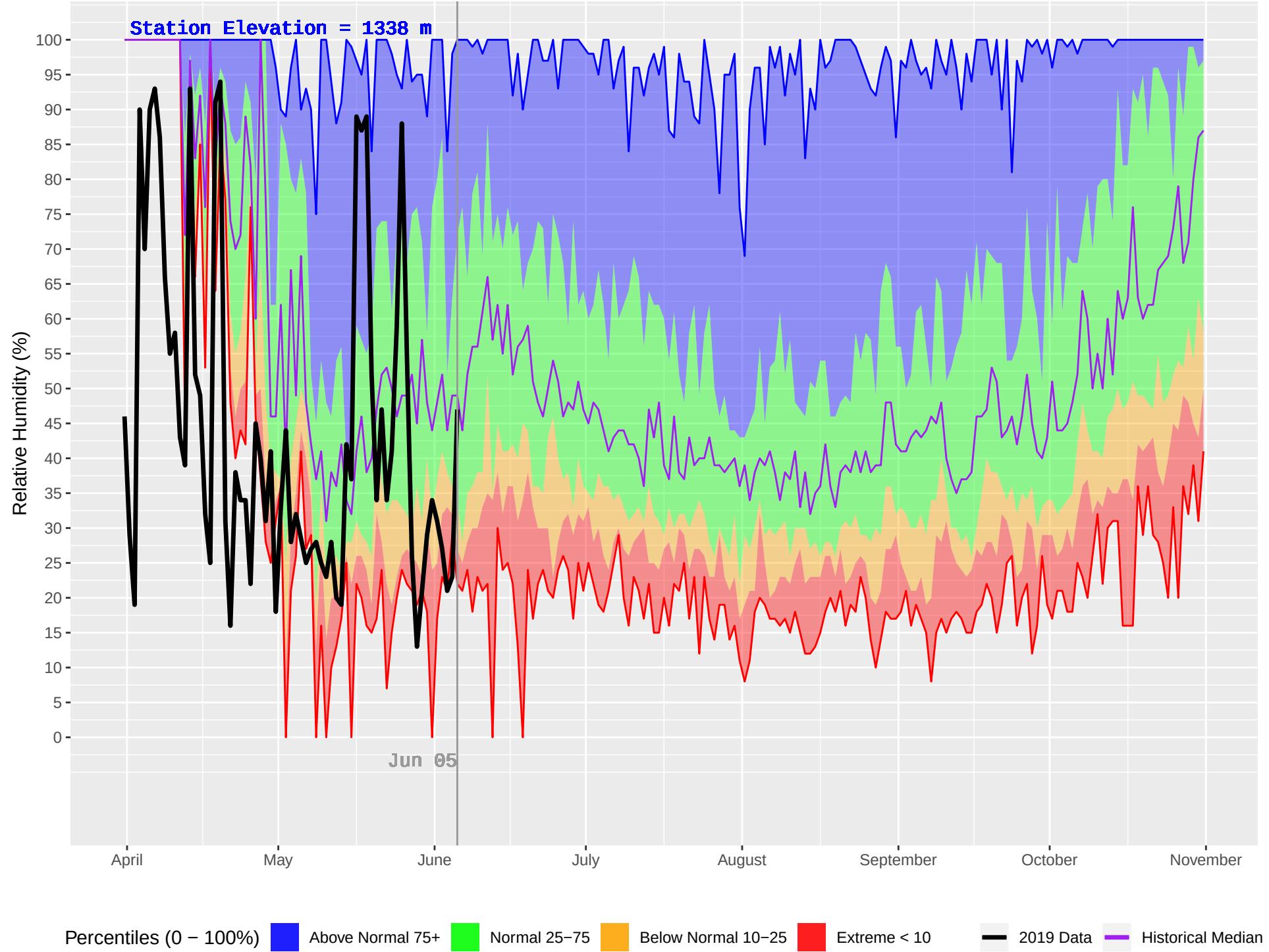
EIGHT MILE (391) : Historical (1980–2018) and Current (2019) Daily Relative Humidity
