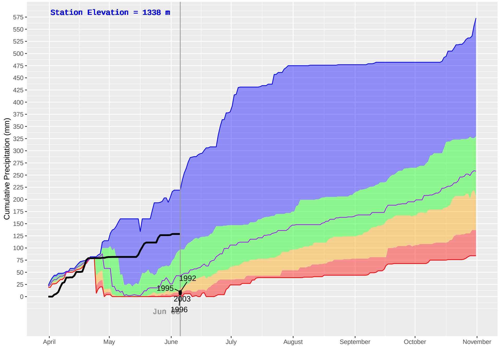
EIGHT MILE (391) : Historical (1980–2018), Current (2019) Daily Cumulative Precipitation
