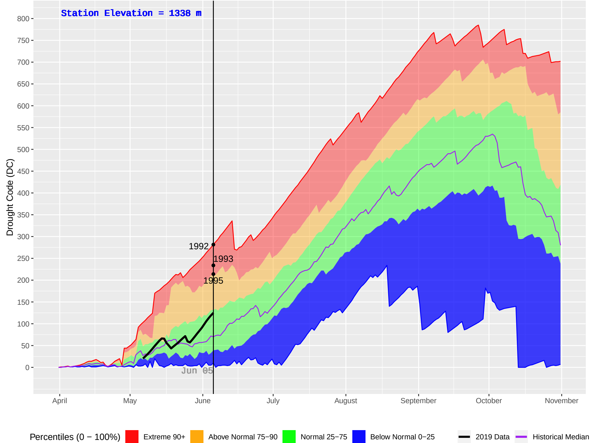
EIGHT MILE (391) : Historical (1980–2018) and Current (2019) Daily Drought Code (DC)
